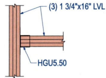
B LVL TO LVL CONNECTION DETAIL SCALE: N.T.S.
