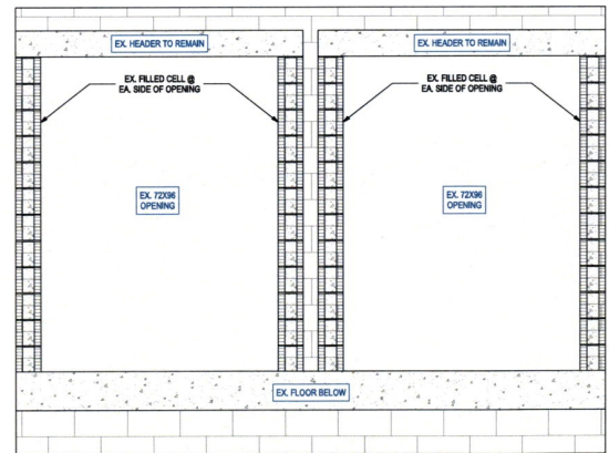
EX. DOOR OPENING VIEW FROM EXTERIOR SCALE: N.T.S.
