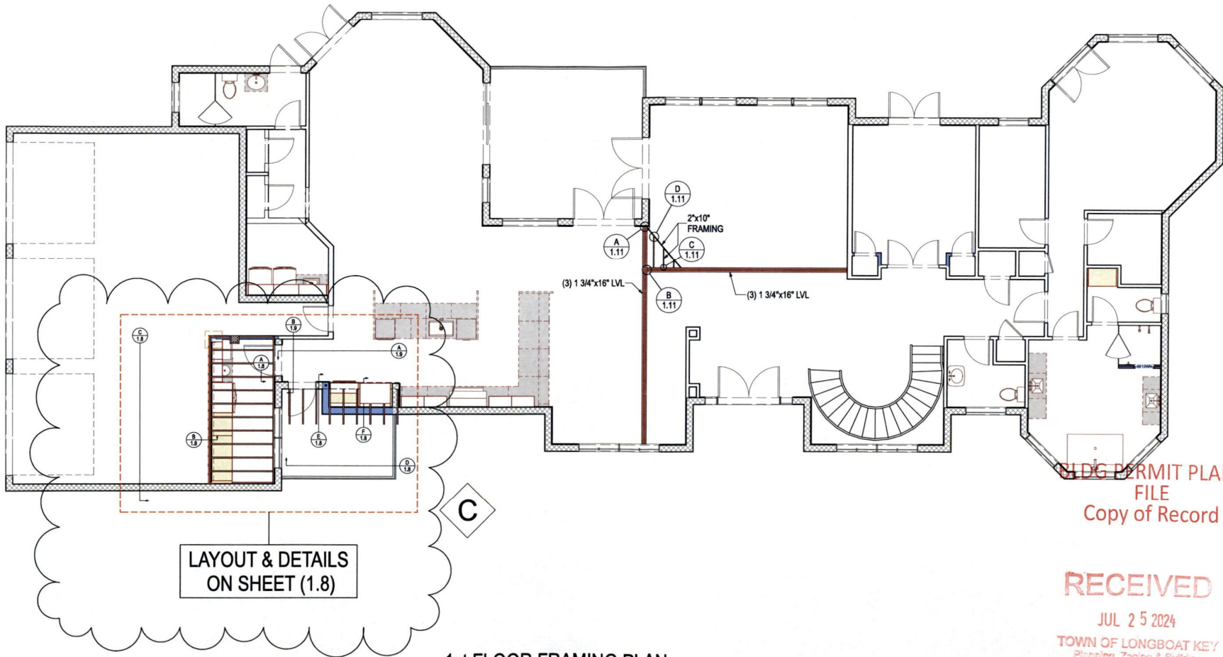
1st FLOOR FRAMING PLAN
