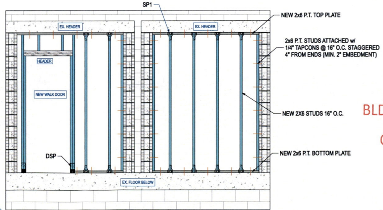
C NEW DOOR OPENING VIEW FROM EXTERIOR SCALE: N.T.S.
