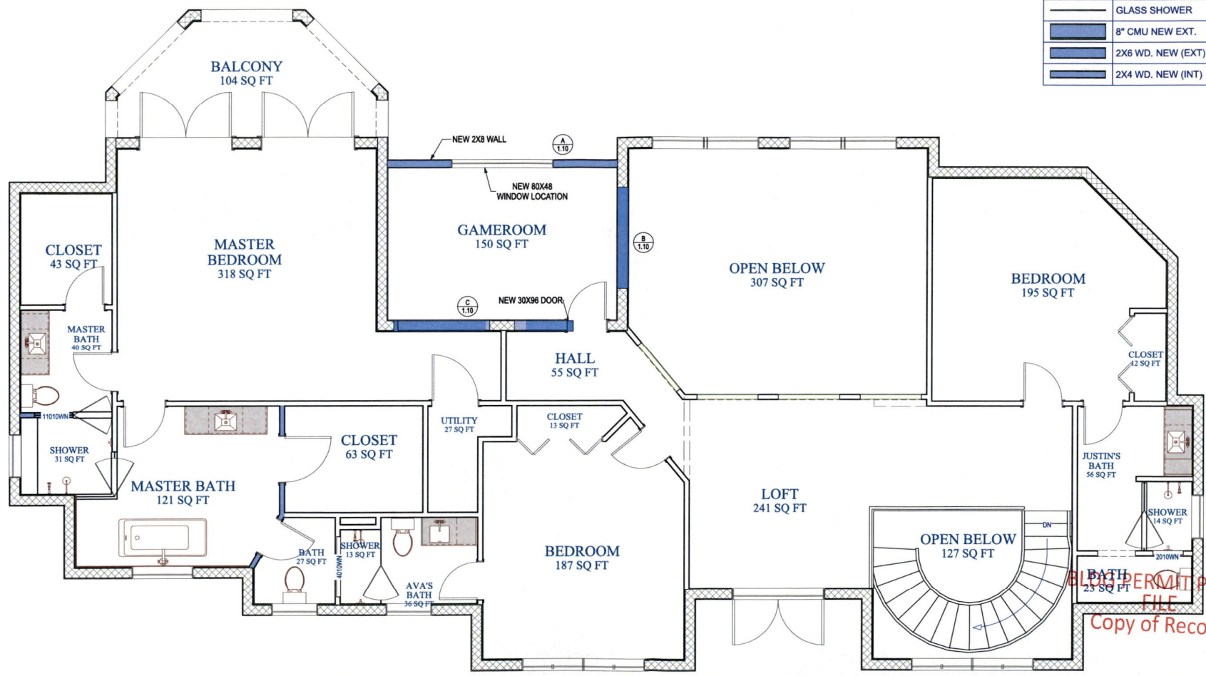
2nd FLOOR PROPOSED FLOOR PLAN
