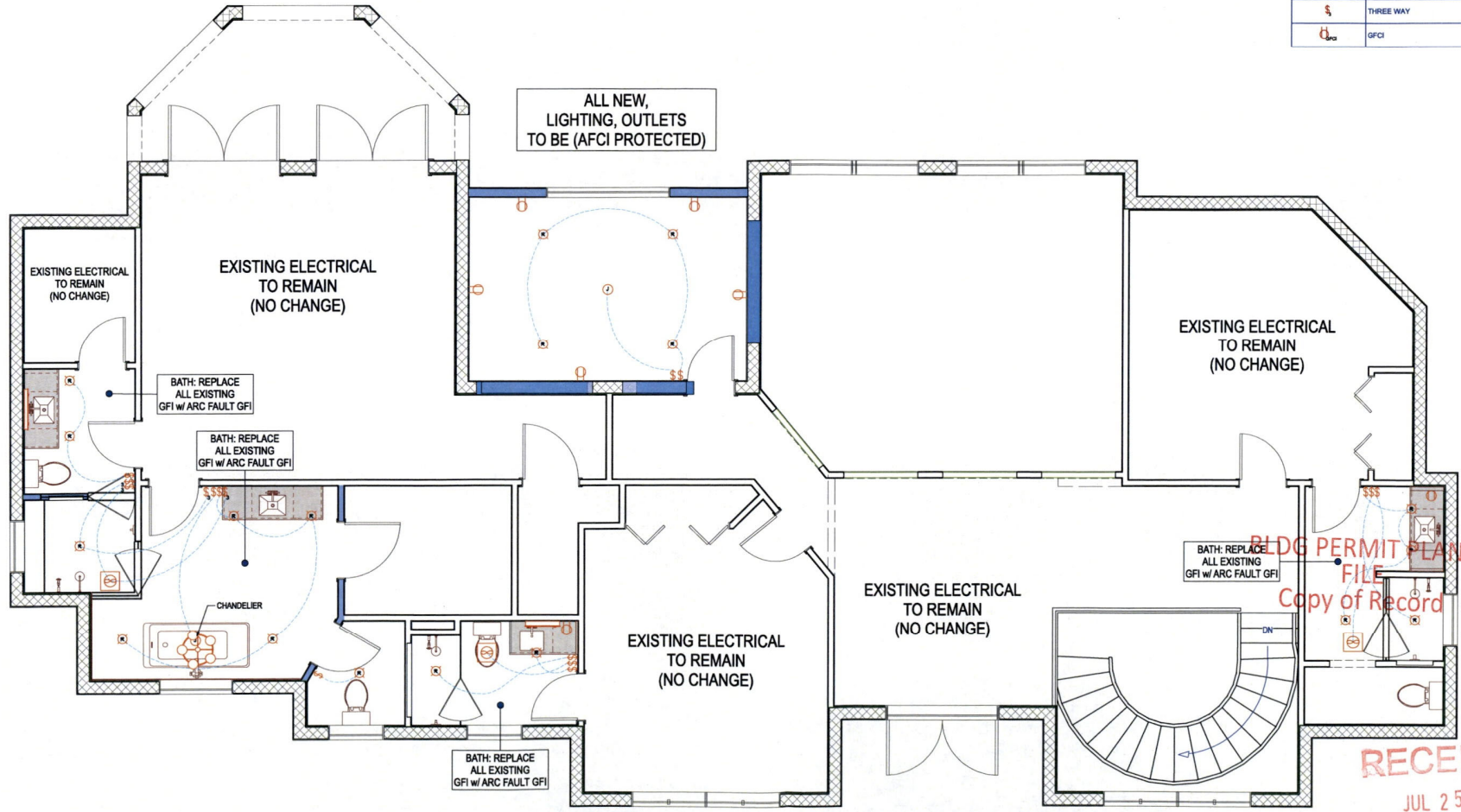
2ND FLOOR ELECTRICAL PLAN
