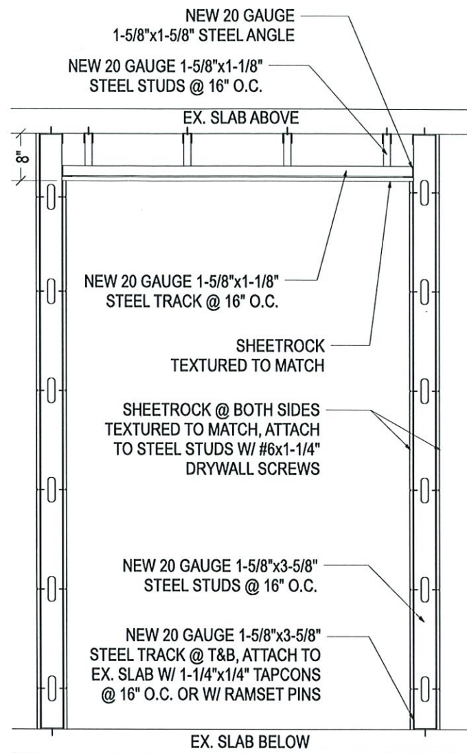
TYP. INTERIOR WALL FRAMING SCALE: NTS
