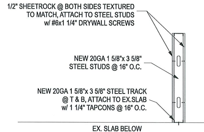
KNEE WALL DETAIL SCALE: NTS
