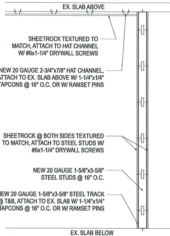
TYPICAL INTERIOR WALL DETAIL SCALE: NTS
