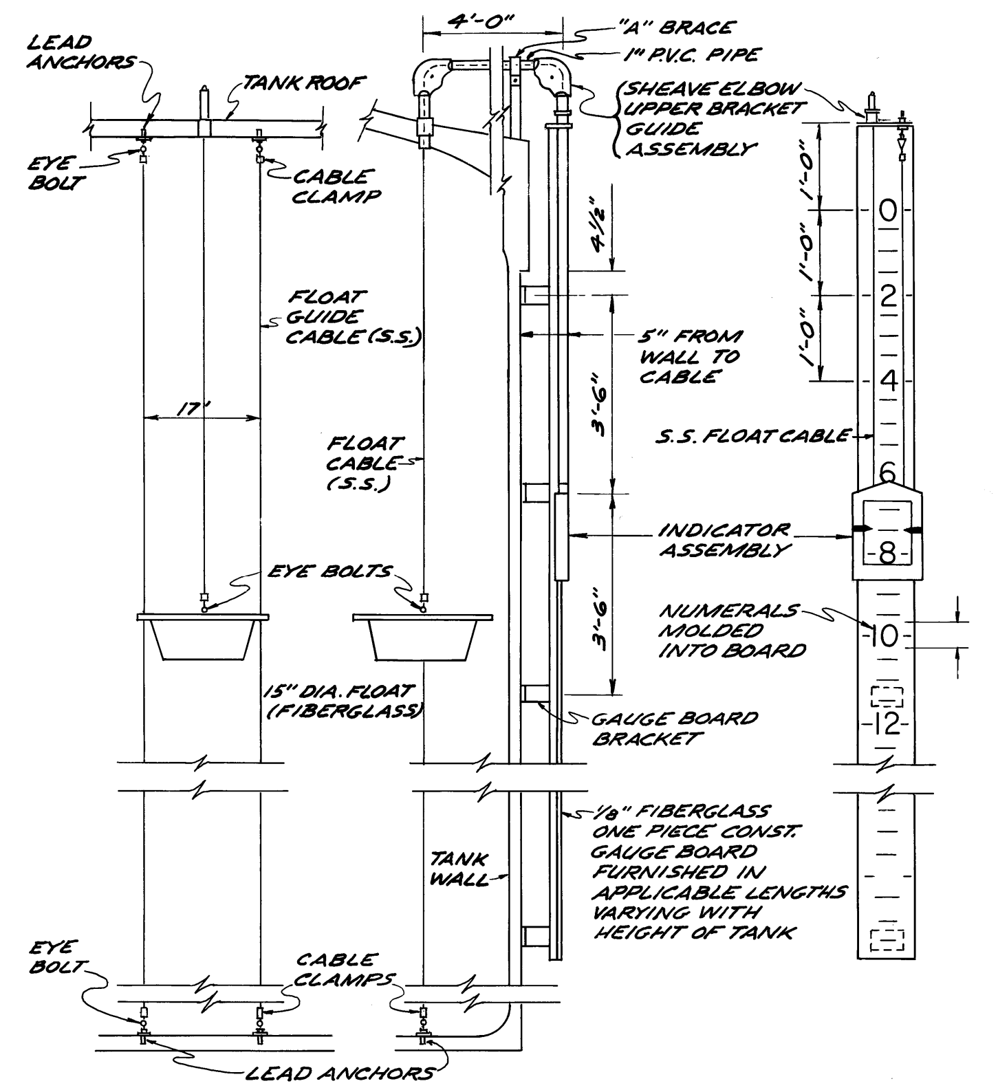
REAR SIDE TRAVEL BOARD LIQUID LEVEL INDICATOR ASSEMBLY NOT TO SCALE
