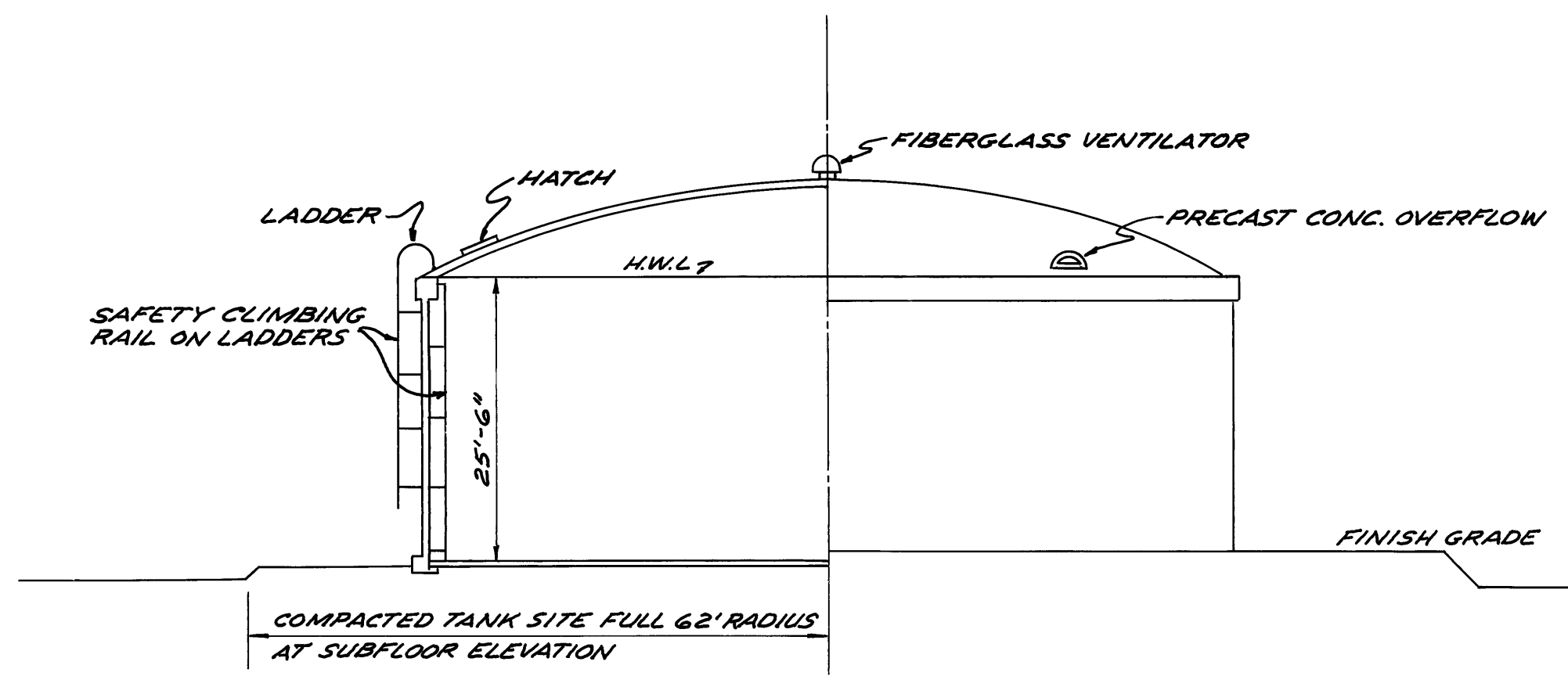
SECTION ELEV. NOT TO SCALE
