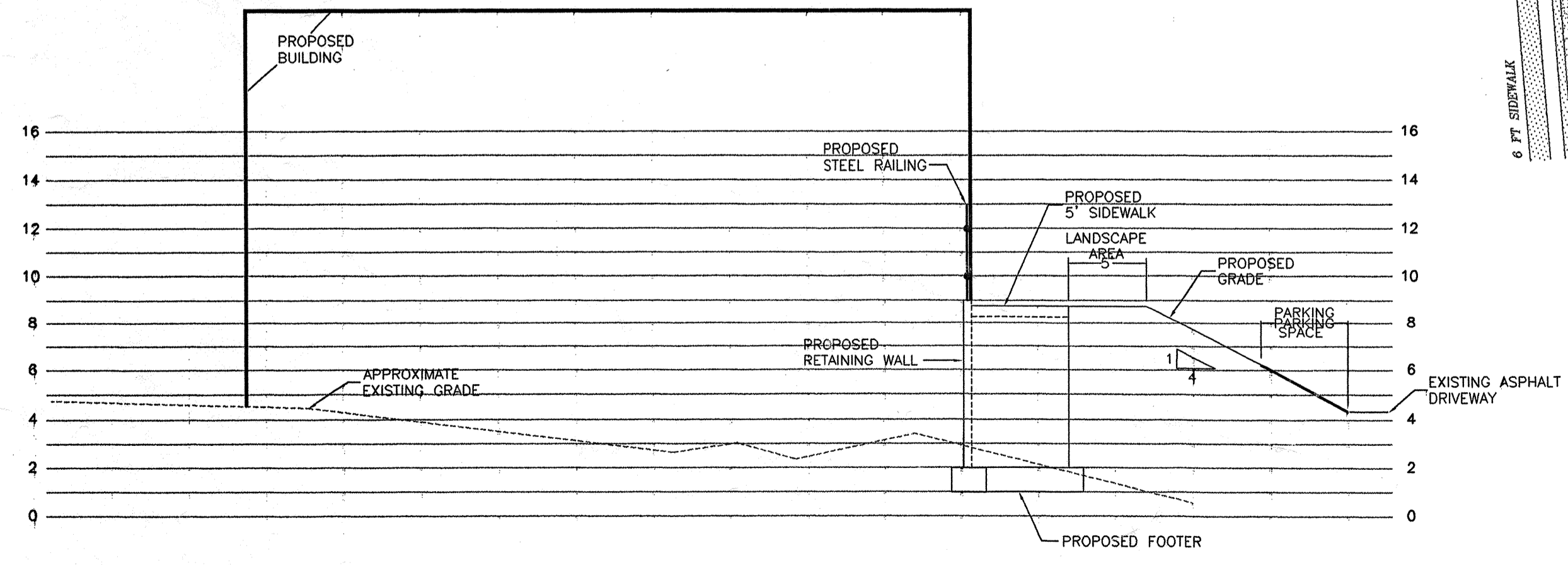
SECTION A-A SCALE: 1"=10' HORIZONTAL 1"=5' VERTICAL
