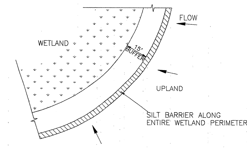
DETAIL 1
