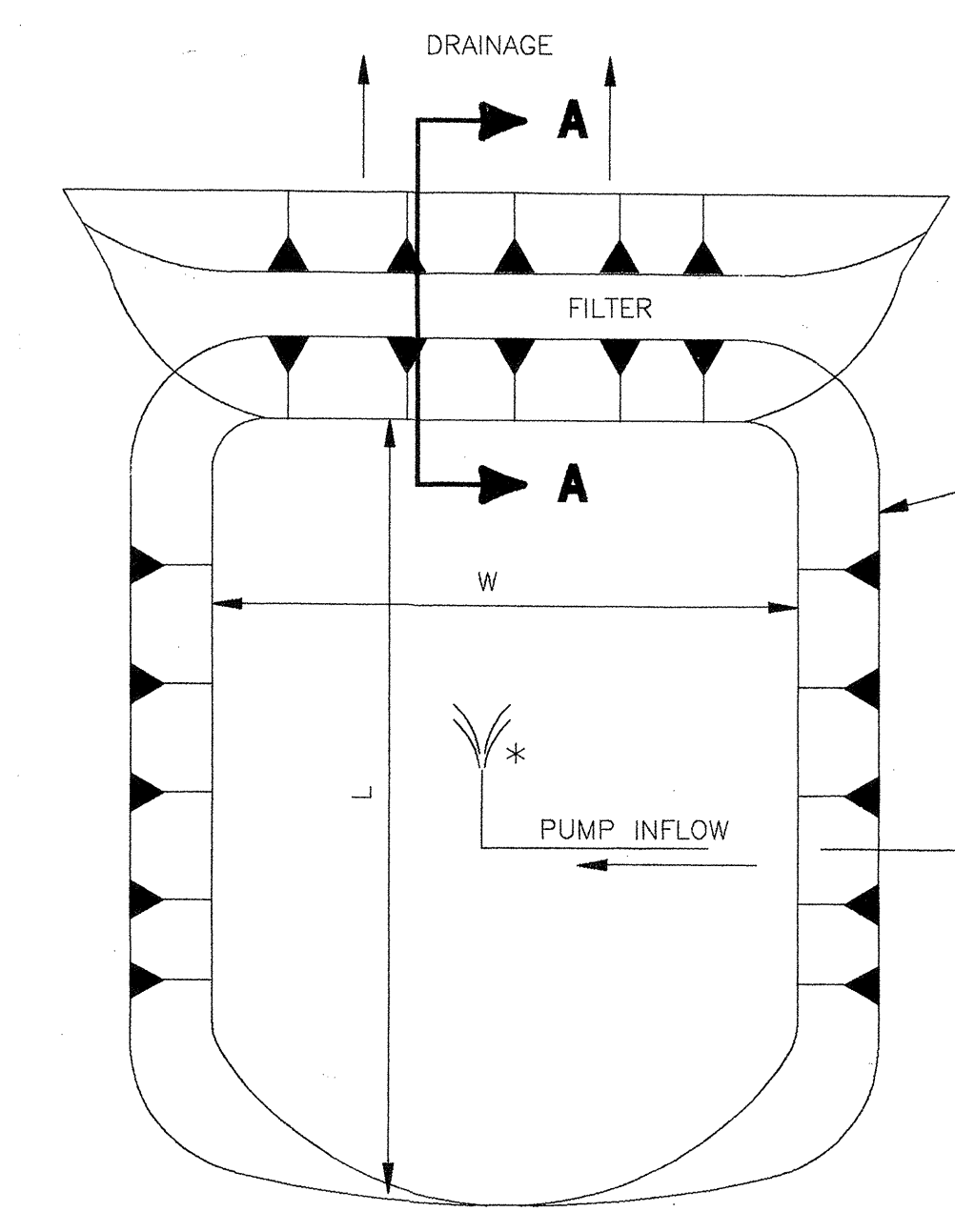
DEWATERING SEDIMENT AND EROSION CONTROL SUMP
