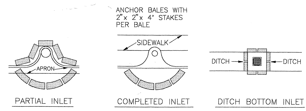
PROTECTION AROUND INLETS
