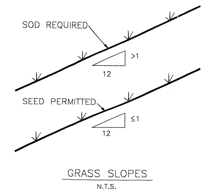
DETAIL 4
