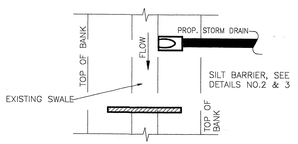
SILT BARRIER AT CONNECTION OF STORM PIPE TO EXISTING SWALE
