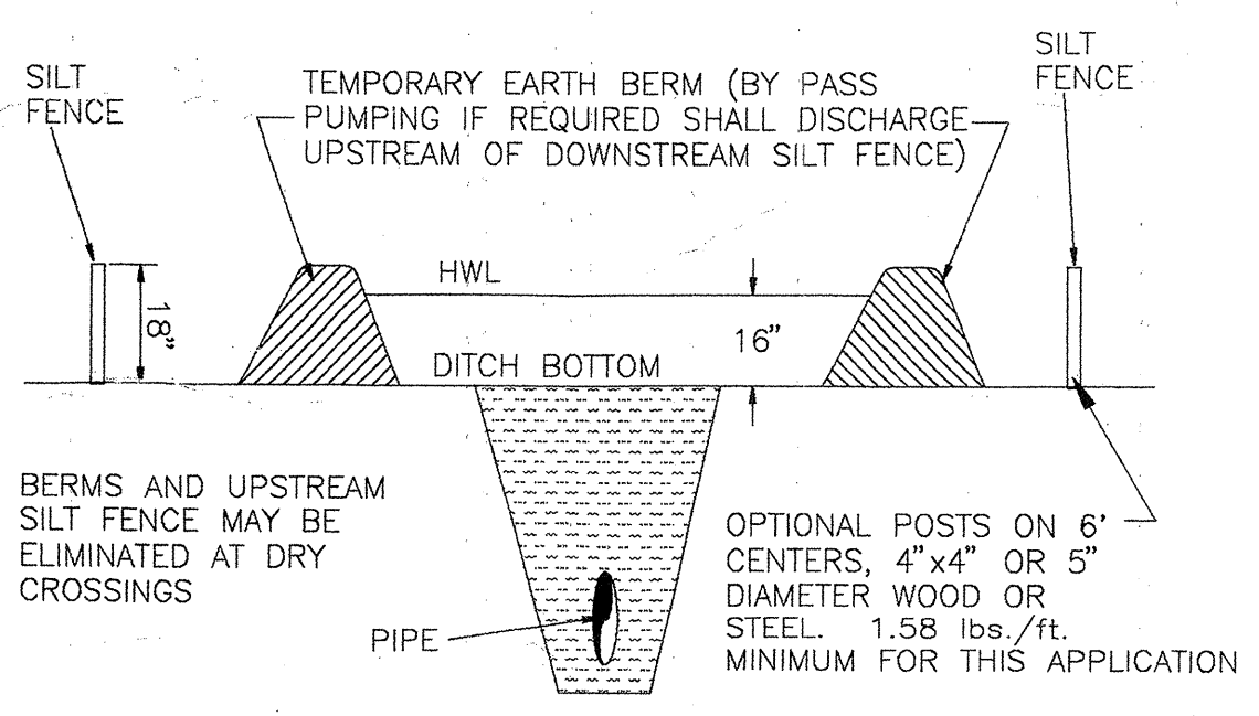
UNDERGROUND PIPE CROSSINGS
