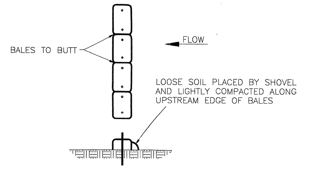
DETAIL 3
