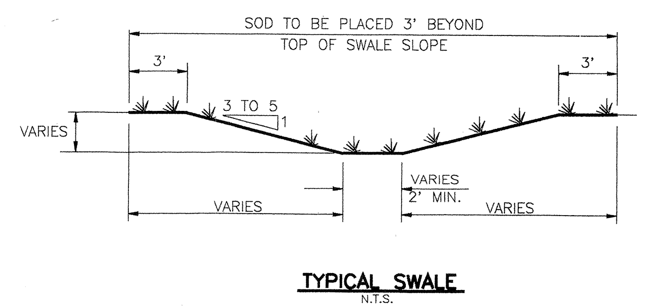
DETAIL 5
