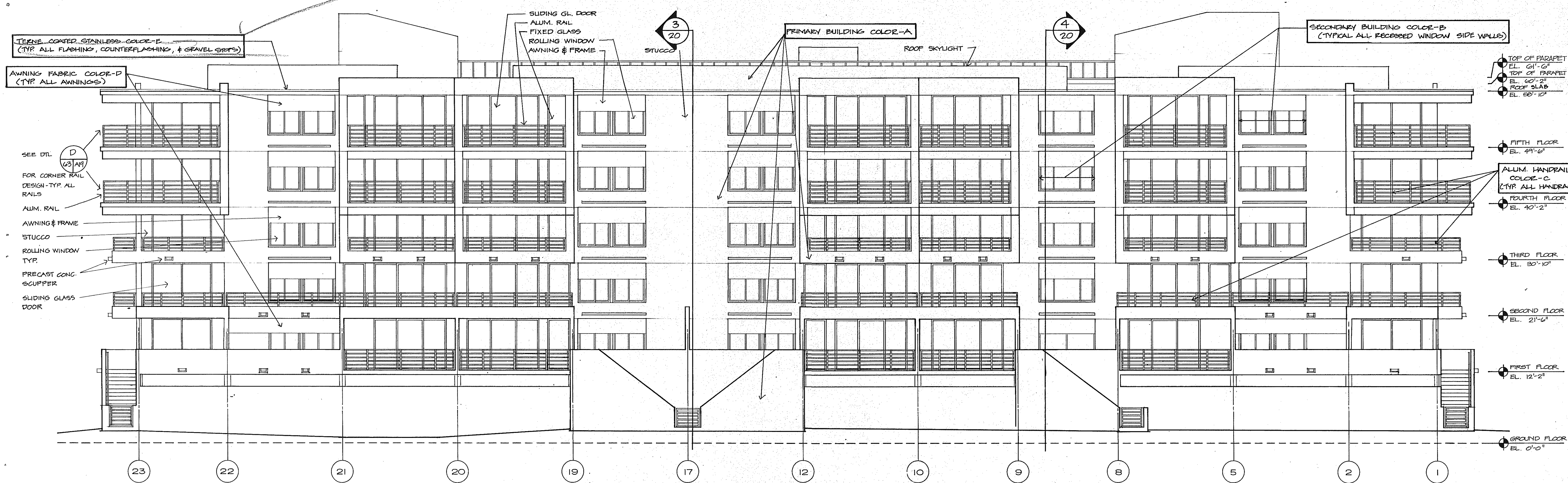
BEACH ELEVATION 1/19
