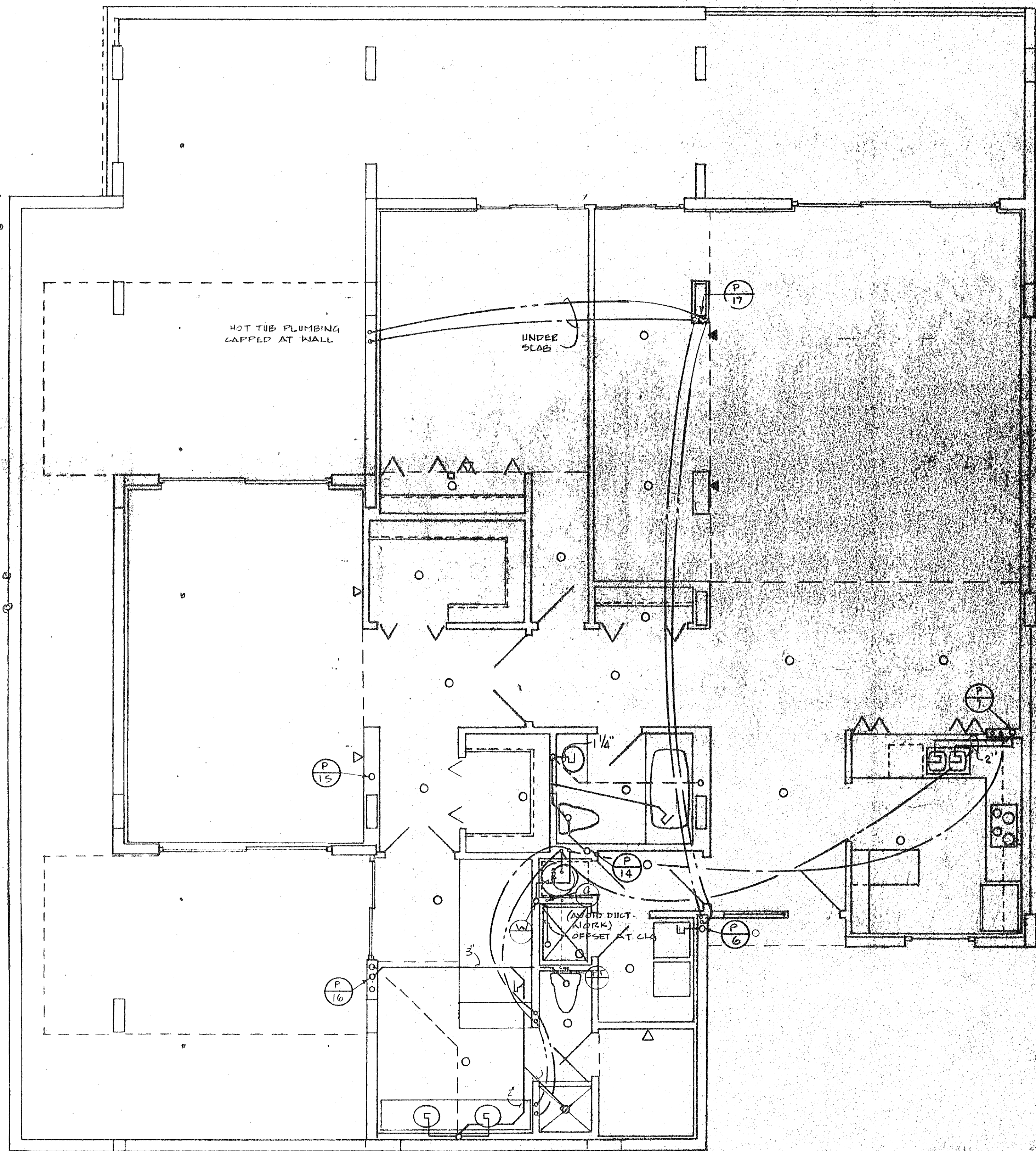
UNIT D4 LEFT PLUMBING PLAN
