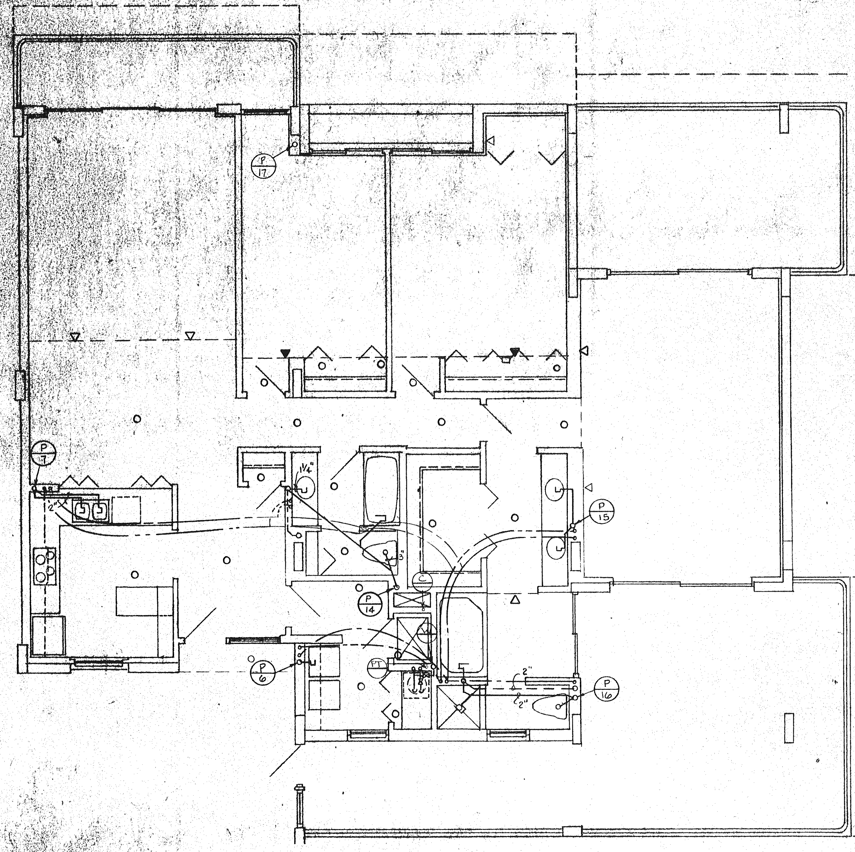
UNIT 'D' RIGHT - PLUMBING PLAN
