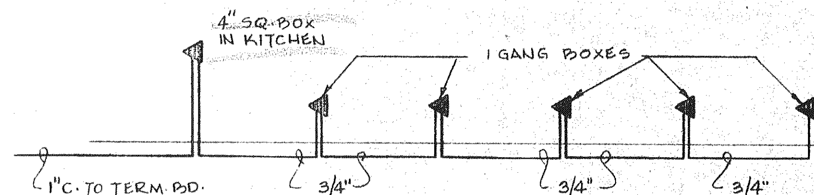
THREE BEDROOM APARTMENT RISER DIAGRAM
