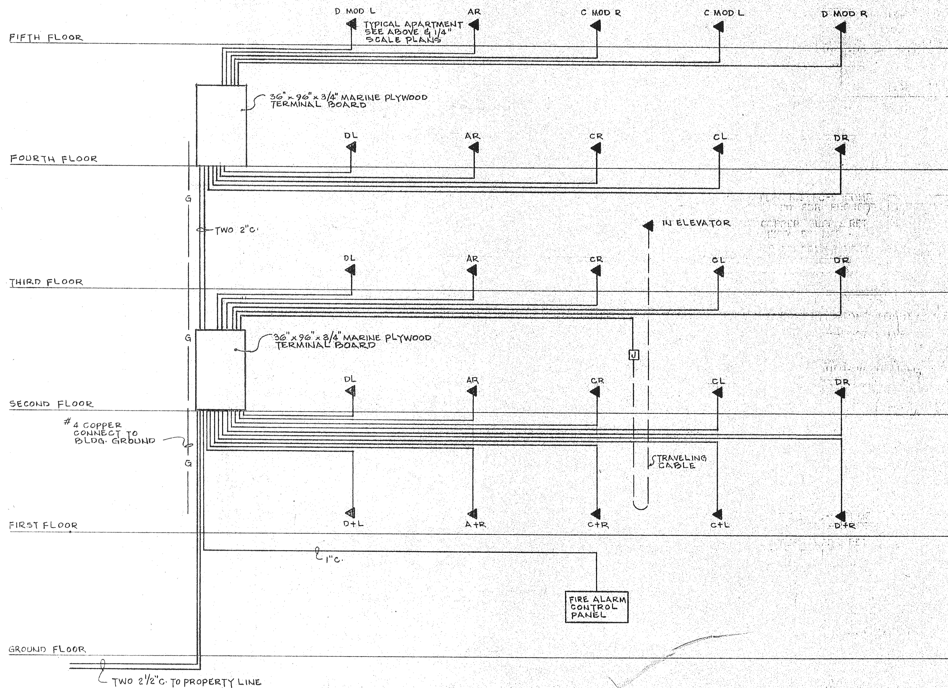
BUILDING 3 - TELEPHONE RISER DIAGRAM
