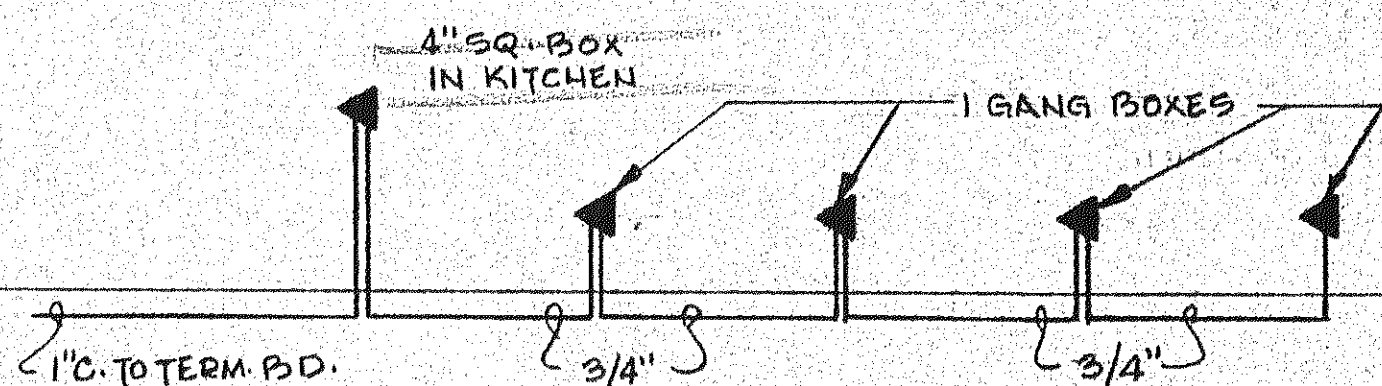
TWO BEDROOM APARTMENT RISER DIAGRAM
