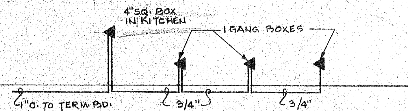
ONE BEDROOM APARTMENT RISER DIAGRAM
