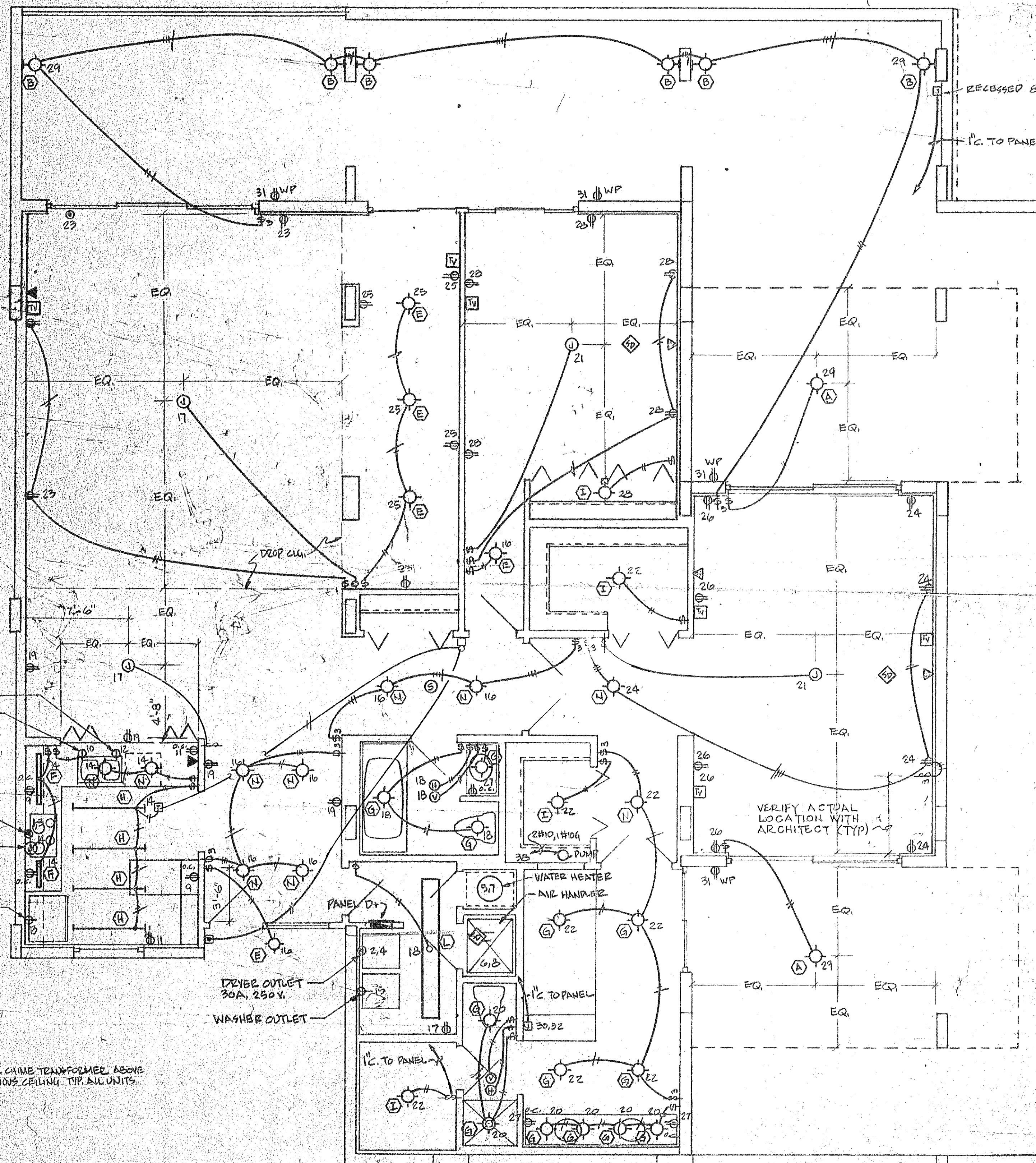
UNIT D+ RIGHT ELECTRICAL PLAN
