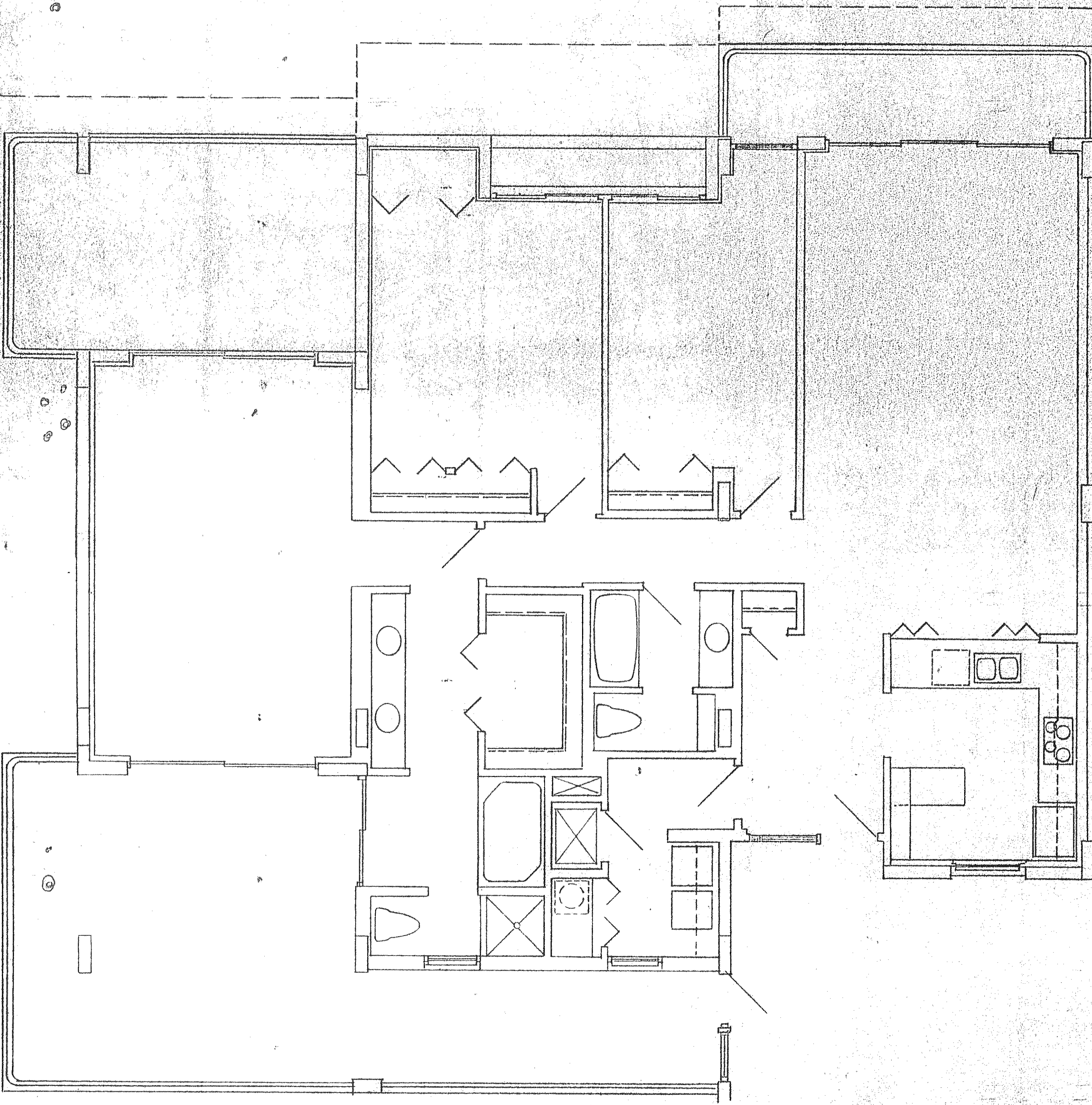
UNIT 'D' LEFT SCALE 1/4" = 1'-0"
