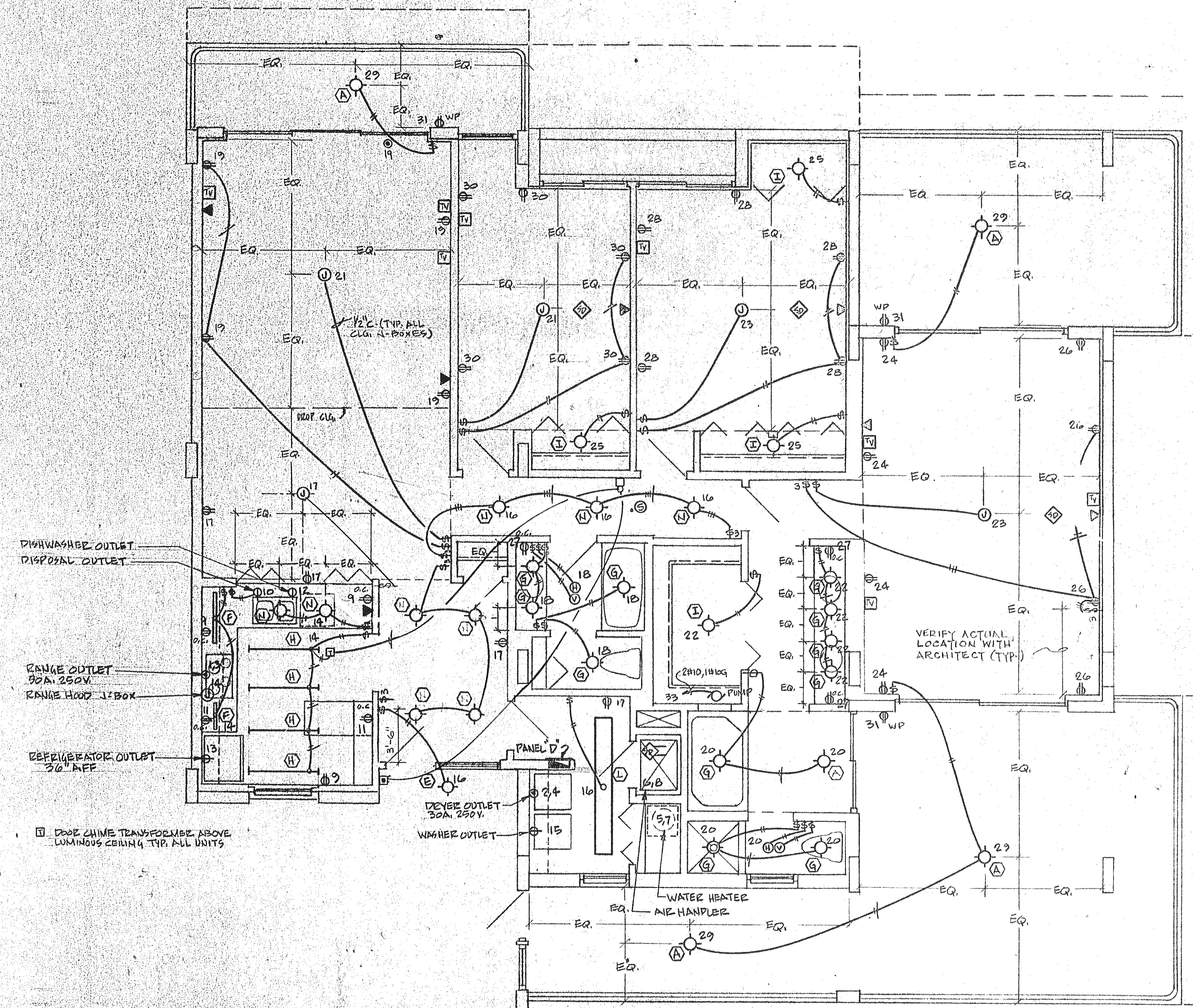
UNIT 'D' RIGHT - ELECTRICAL PLAN SCALE 1/4" = 1'-0"
