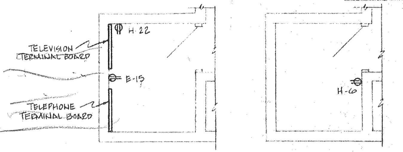
FOURTH FLOOR TEL. & T.V. CLOSET N.T.S. FIFTH FLOOR STORE ROOM N.T.S.
