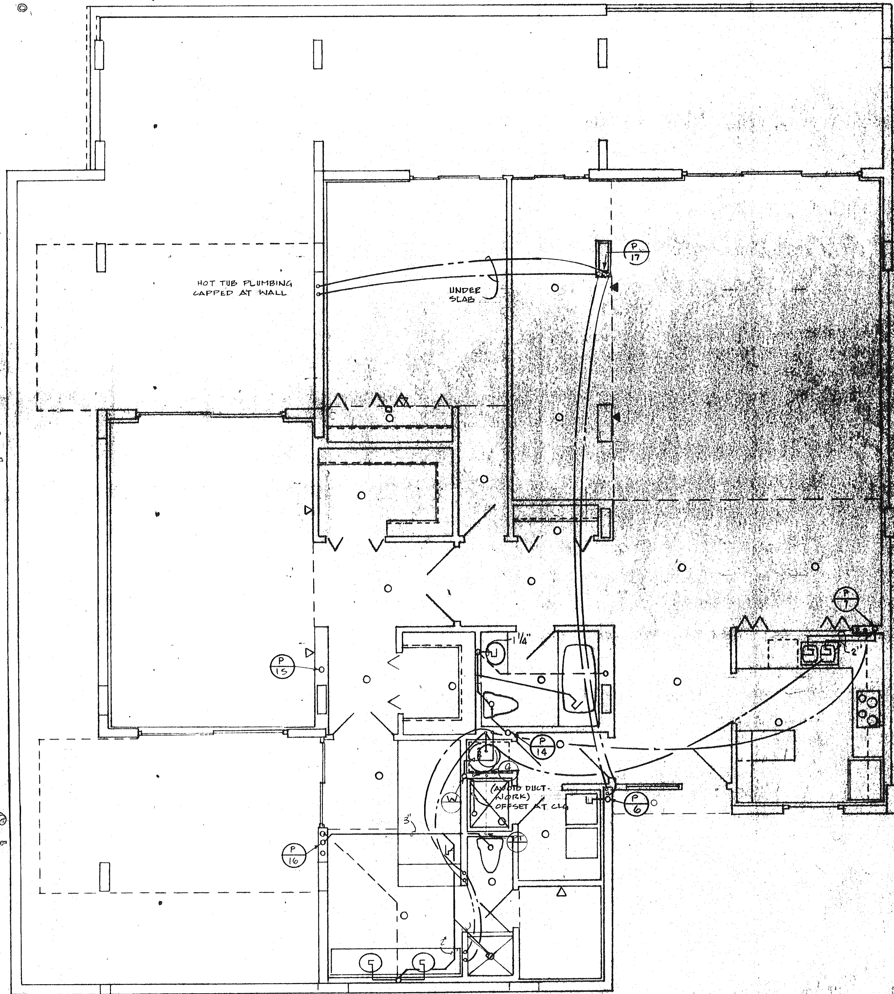
UNIT 04 LEFT PLUMBING PLAN
