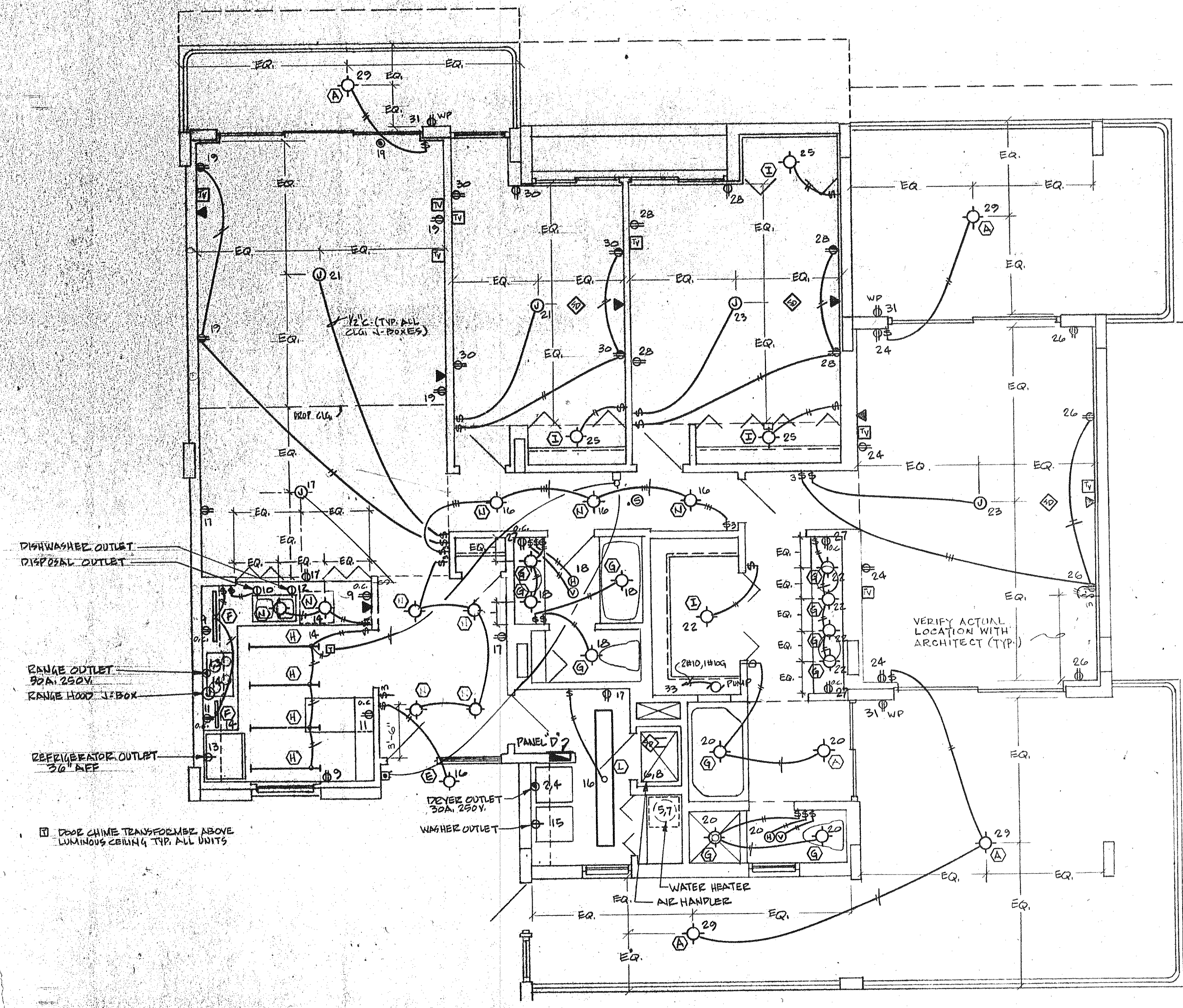
UNIT 'D' RIGHT - ELECTRICAL PLAN 12'0" x 12'0"
