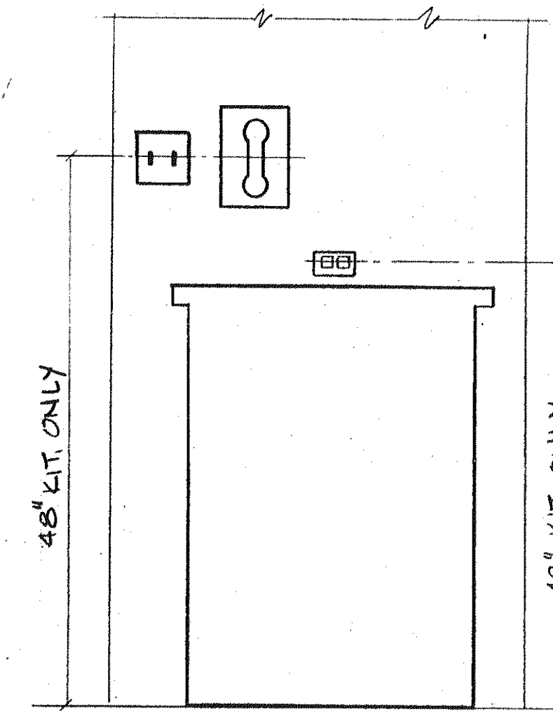
SECTION "B-B" (TYP.) scale 1" : 1'-0"
