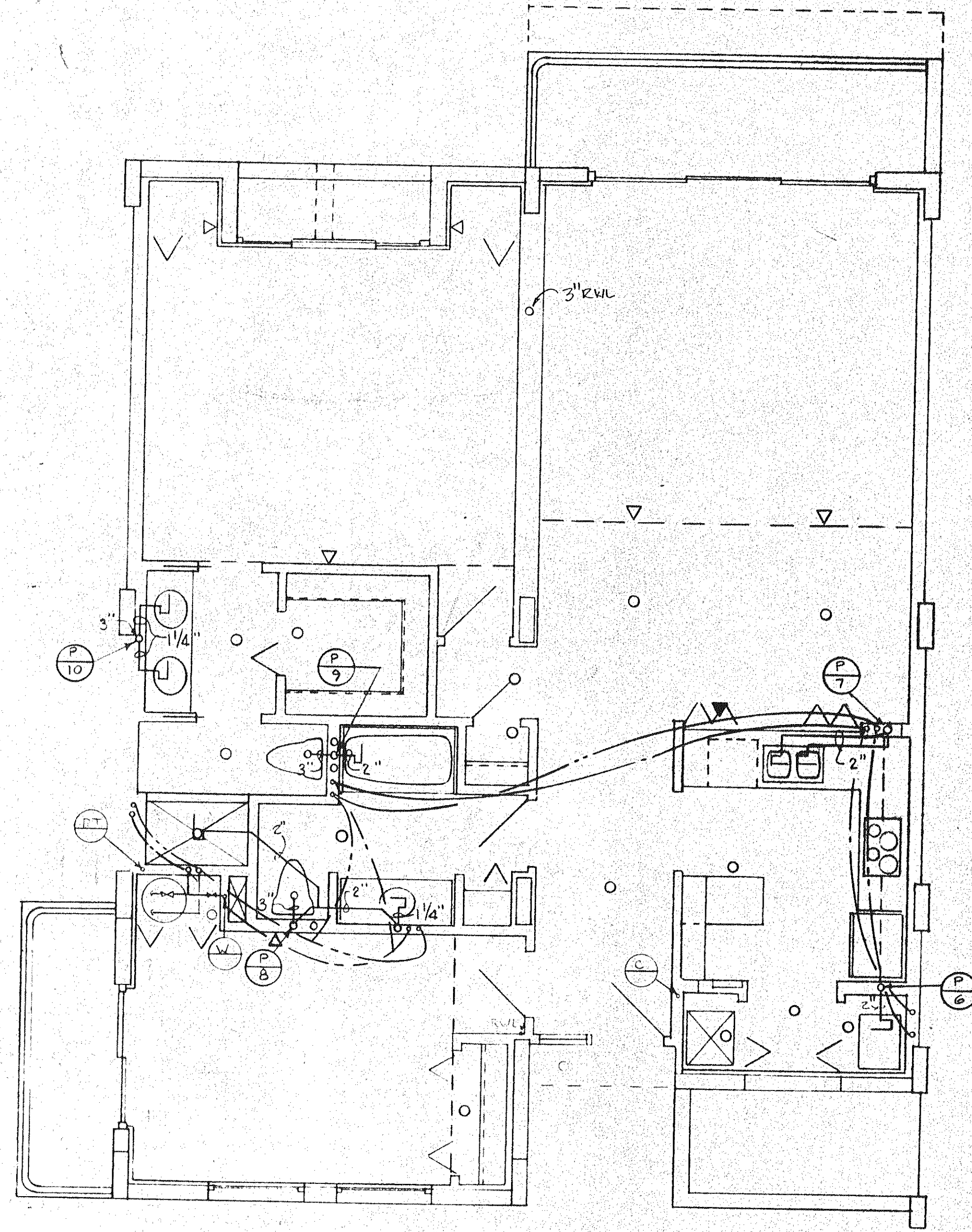
UNIT 'B' LEFT. PLUMBING PLAN
