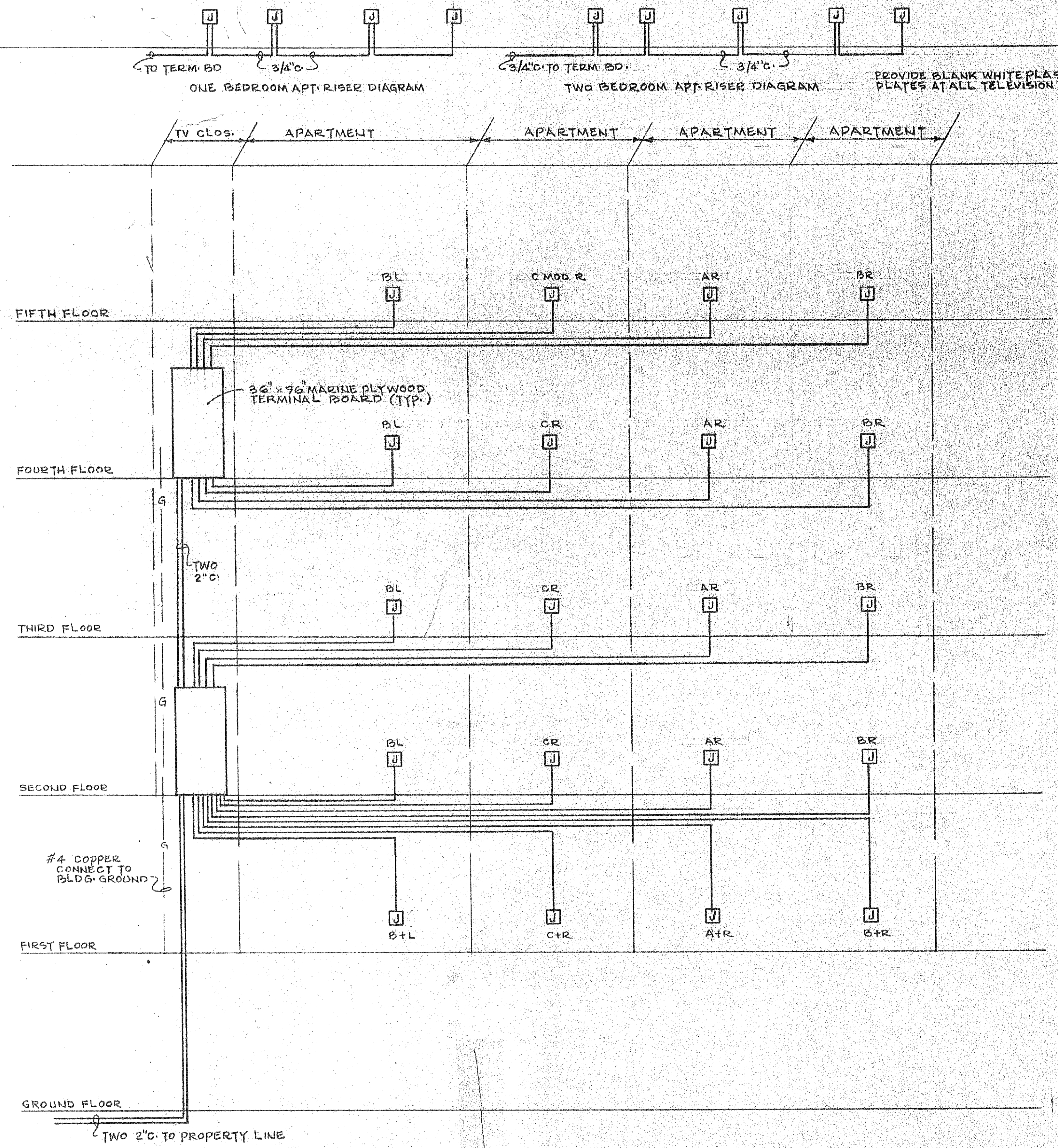
BUILDING 2 TELEVISION RISER DIAGRAM
