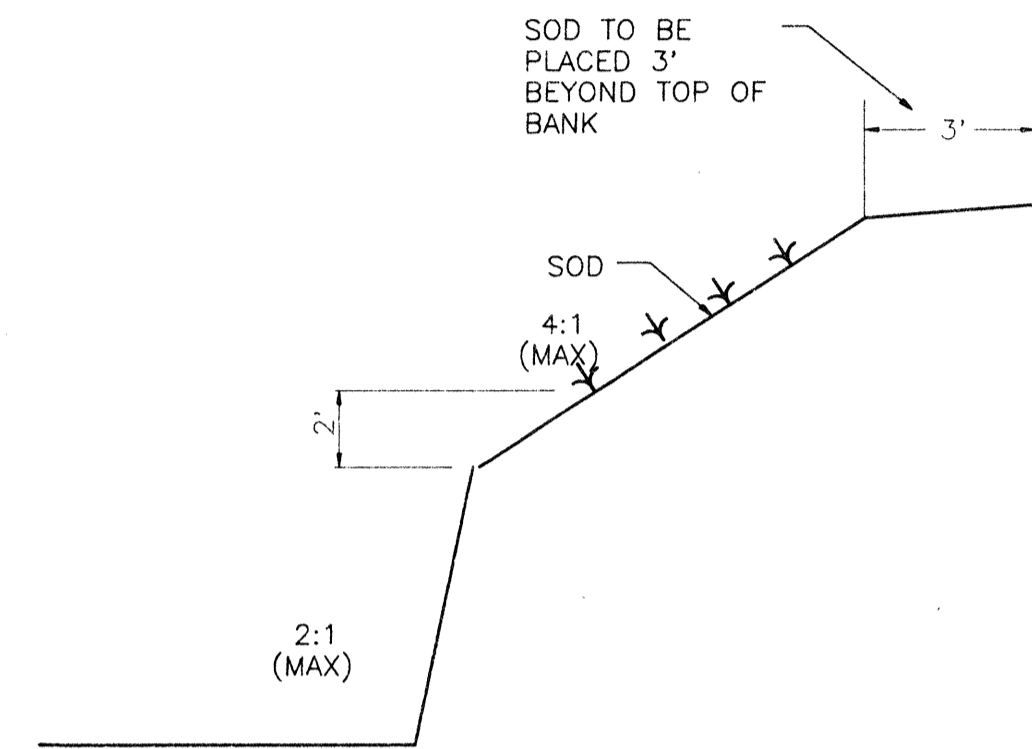
TYPICAL RETENTION/DETENTION POND SECTION N.T.S.
