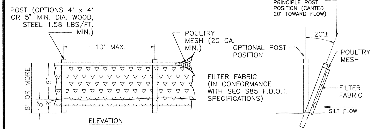
TYPICAL SILT FENCE N.T.S.
