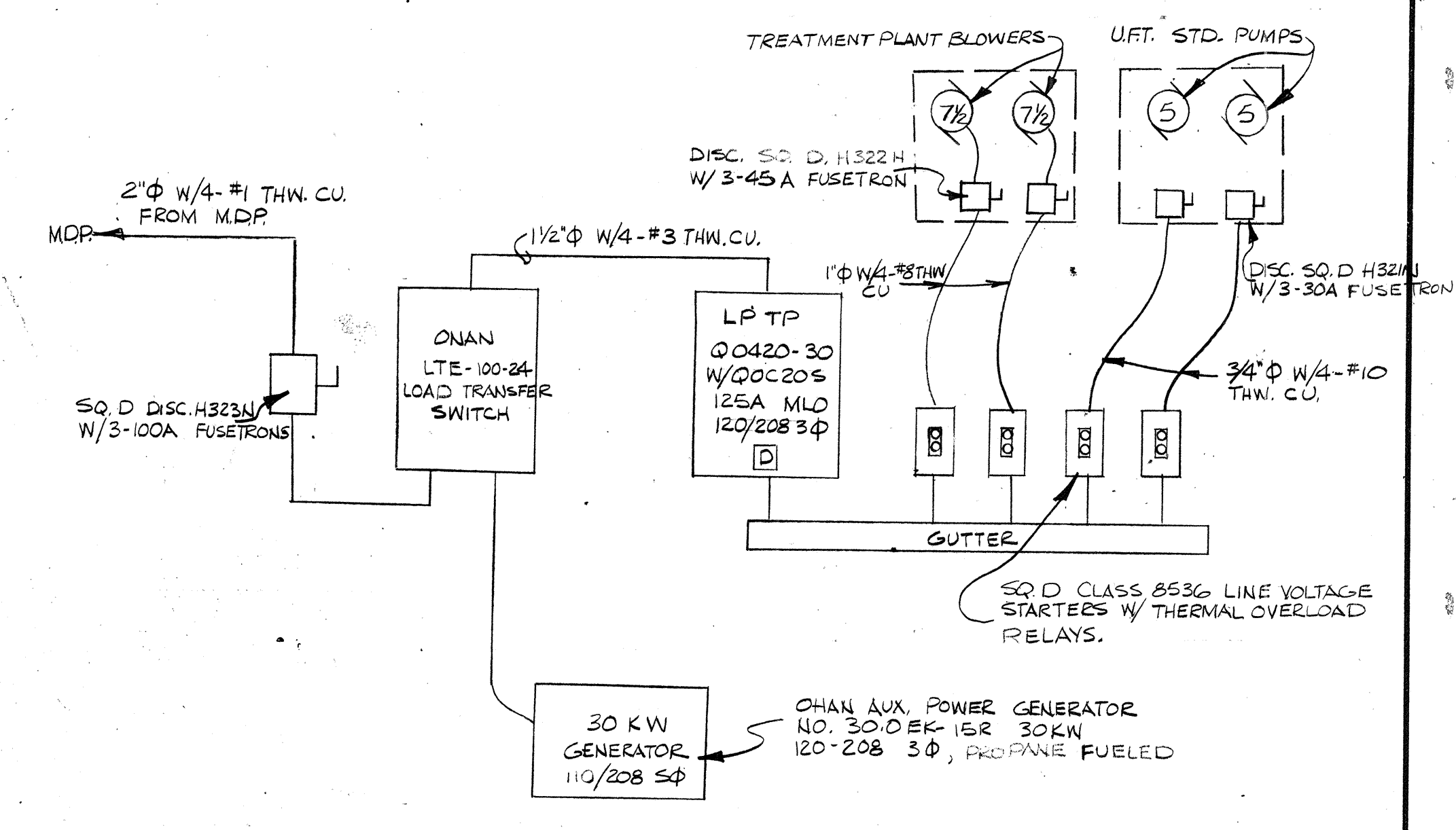
TREATMENT PLANT ELECTRICAL DIAGRAM
