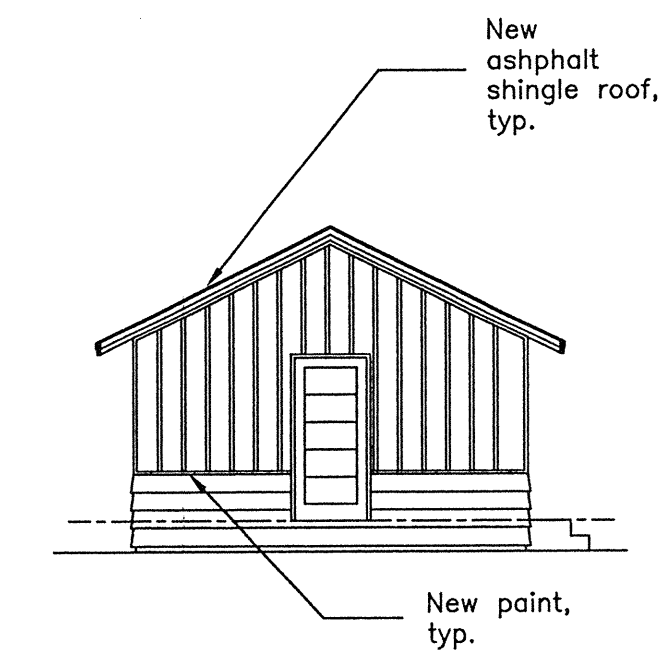
SOUTH ELEVATION
