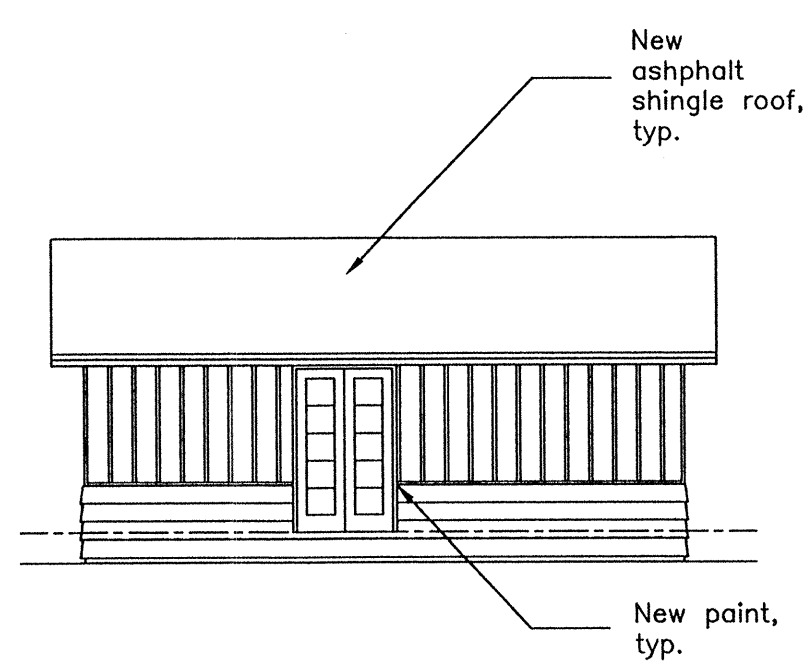
EAST ELEVATION
