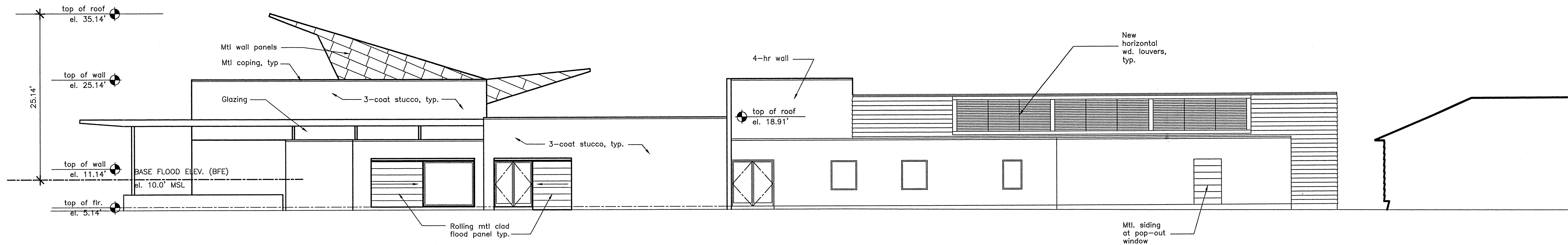
WEST ELEVATION
